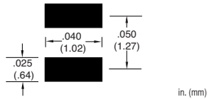
RECOMMENDED FOOT PRINT
