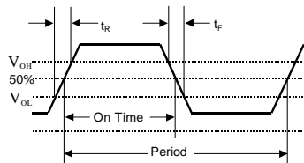
Figure 7. Output Waveform
